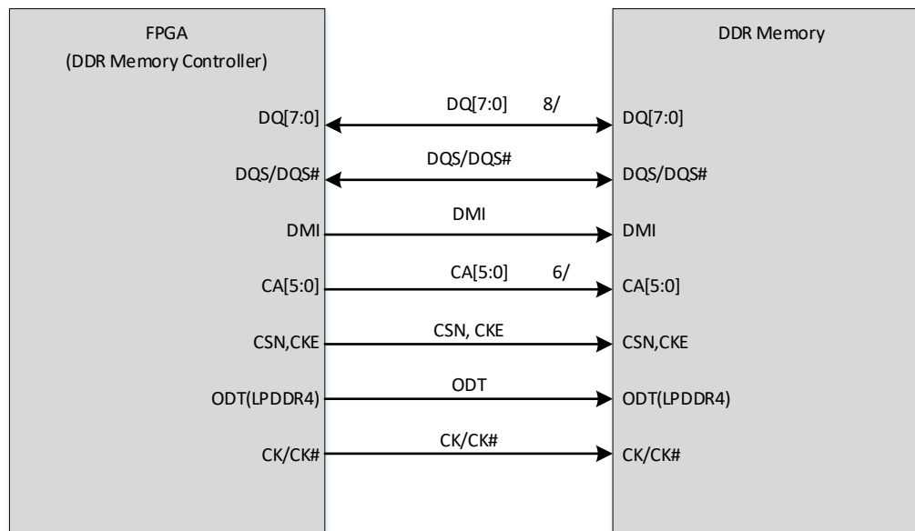
Figure 6.3. Typical LPDDR4 Memory Interface
