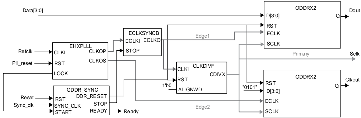
Figure 5.39. GDDR2_TX.ECLK.Centered Interface
