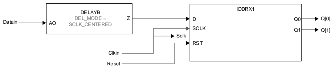
Figure 5.11. GDDR1_RX.SCLK.Centered Interface (Static Delay)
