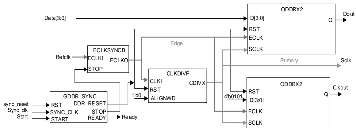
Figure 5.38. GDDR2_TX.ECLK.Aligned Interface
