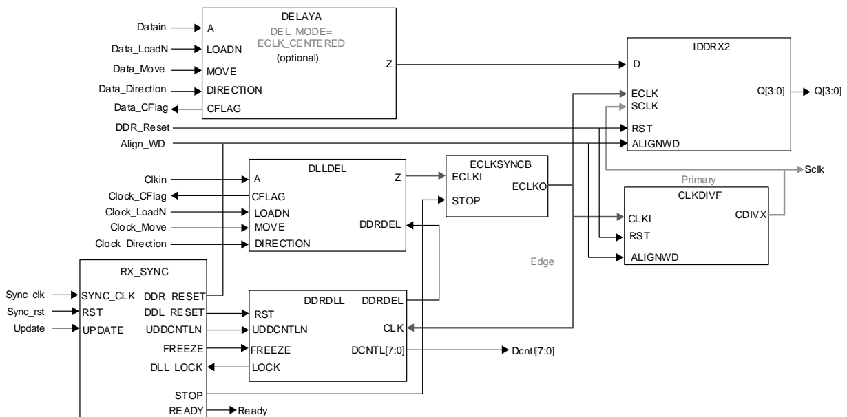
Figure 5.18. GDDR2_RX.ECLK.Aligned Interface (Dynamic Data/Clock Delay)
