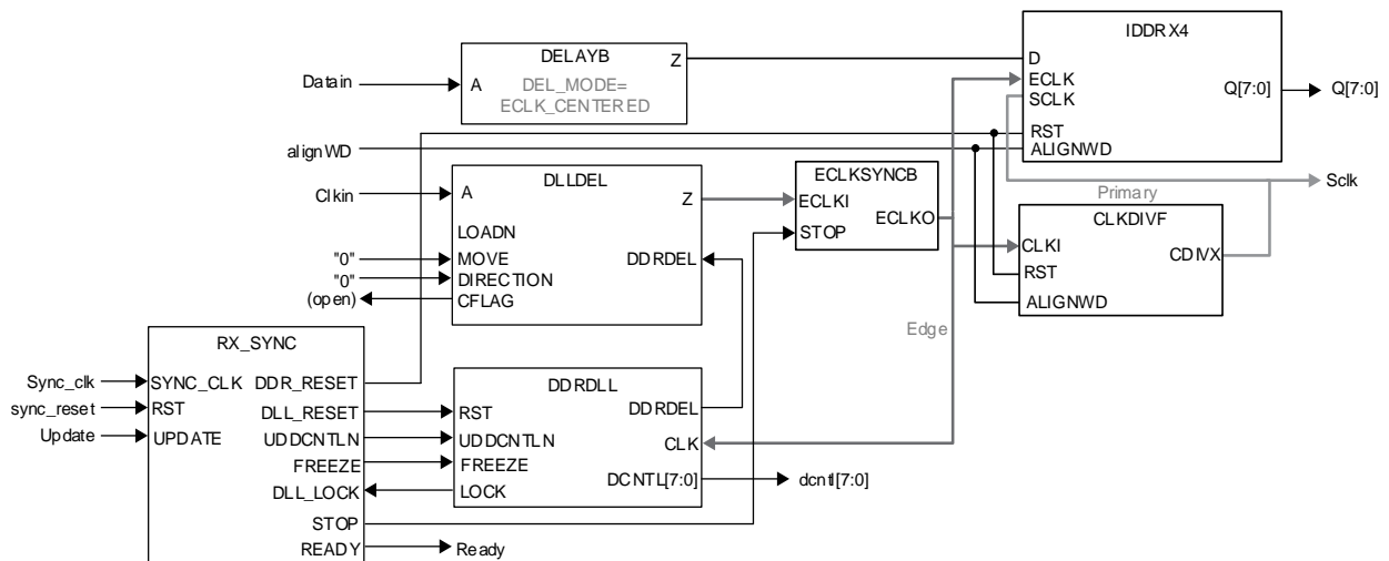
Figure 5.21. GDDR4_RX.ECLK.Aligned Interface (Static Delay)
