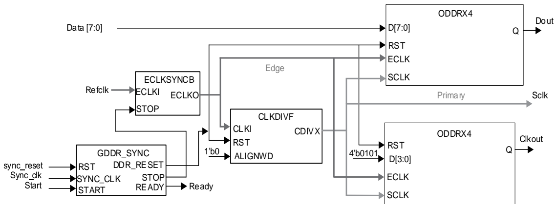
Figure 5.40. GDDR4_TX.ECLK.Aligned Interface
