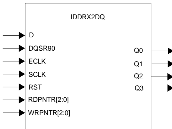
Figure 8.17. IDDRX2DQ Primitive
