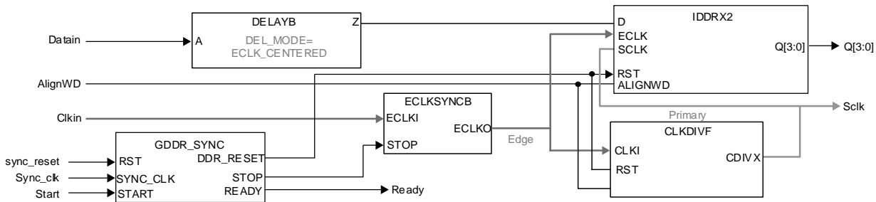
Figure 5.15. GDDR2_RX.ECLK.Centered Interface (Static Delay)
