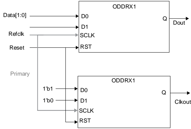
Figure 5.36. GDDR1_TX.SCLK.Aligned Interface
