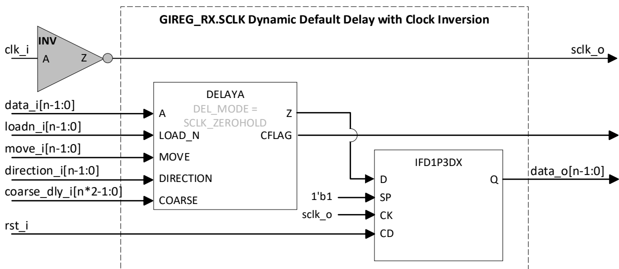
Figure 5.8. GIREG_RX.SCLK (Dynamic Default Delay with Clock Inversion)
