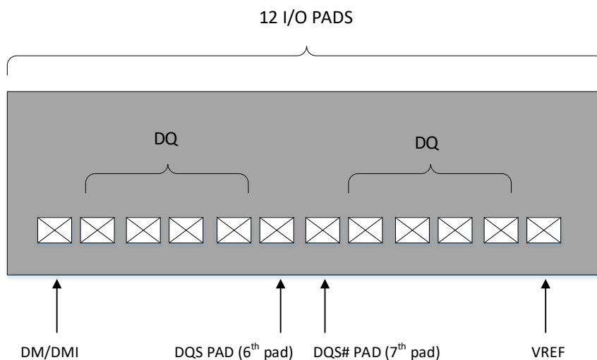
Figure 6.6. DQ-DQS Grouping
