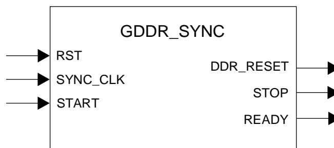
Figure 9.1. GDDR_SYNC Ports
