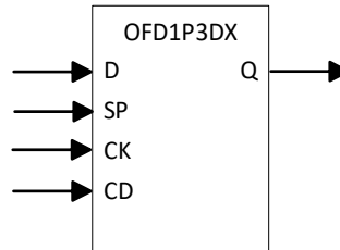
Figure 8.6. OFD1P3DX Primitive
