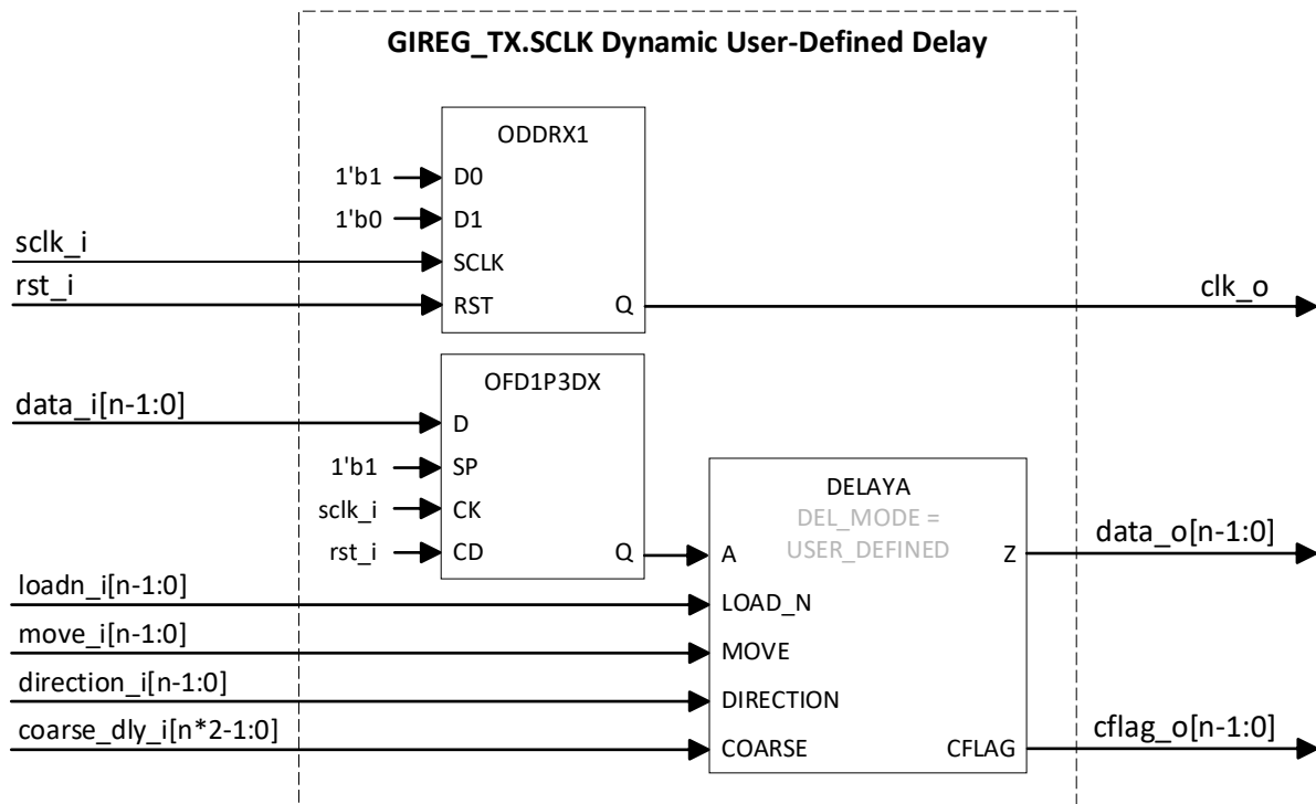
Figure 5.34. GIREG_TX.SCLK (Dynamic User-Defined Delay)
