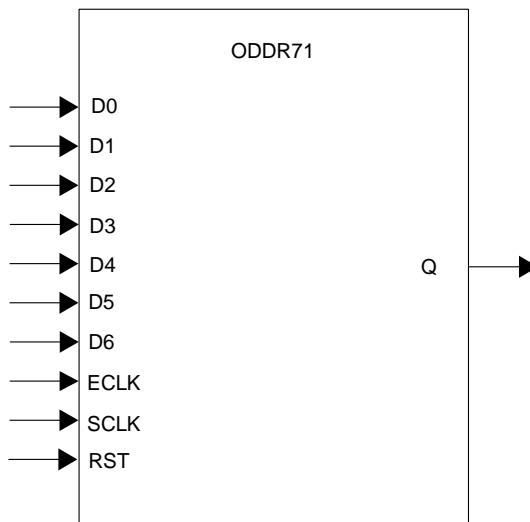
Figure 8.16. ODDR71 Primitive
