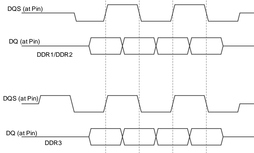
Figure 6.5. DQ-DQS During Write
