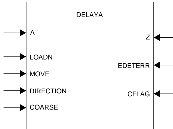
Figure 8.1. DELAYA Primitive
