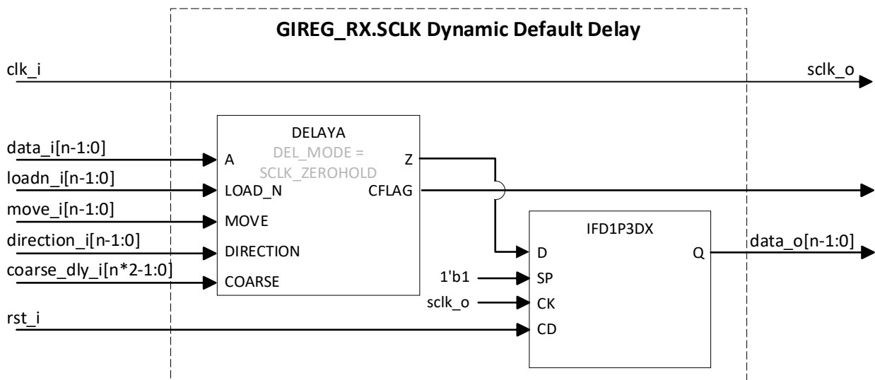
Figure 5.7. GIREG_RX.SCLK (Dynamic Default Delay)
