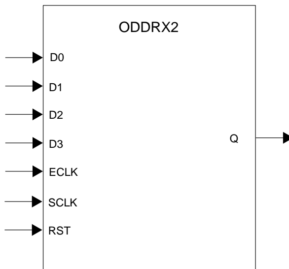
Figure 8.13. ODDR2 Primitive
