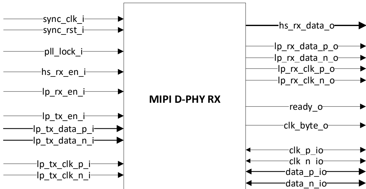
Figure 5.28. MIPI D-PHY RX Block Diagram
