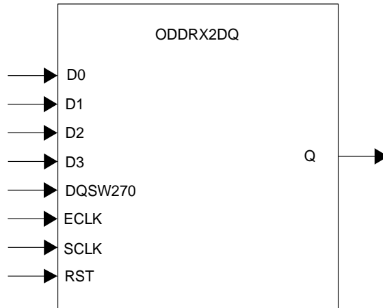
Figure 8.19. ODDR2DQ Primitive
