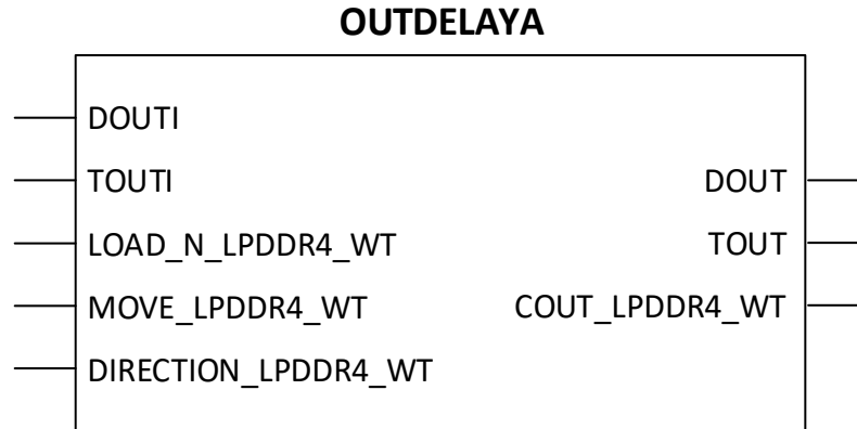
Figure 8.29. OUTDELAYA Primitive
