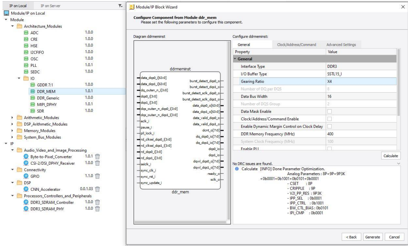
Figure 7.9. DDR_MEM Configuration
