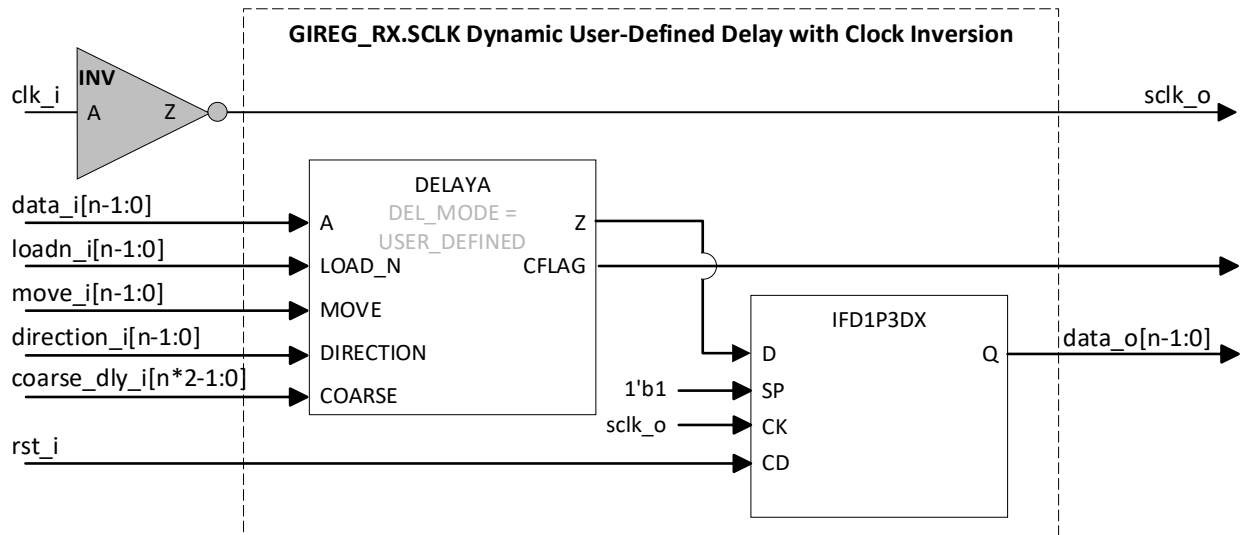
Figure 5.10. GIREG_RX.SCLK (Dynamic User-Defined Delay with Clock Inversion)
