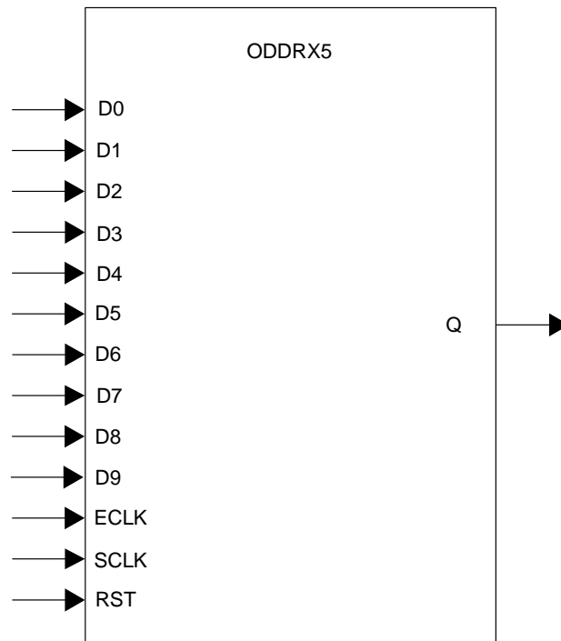
Figure 8.15. ODDR5 Primitive
