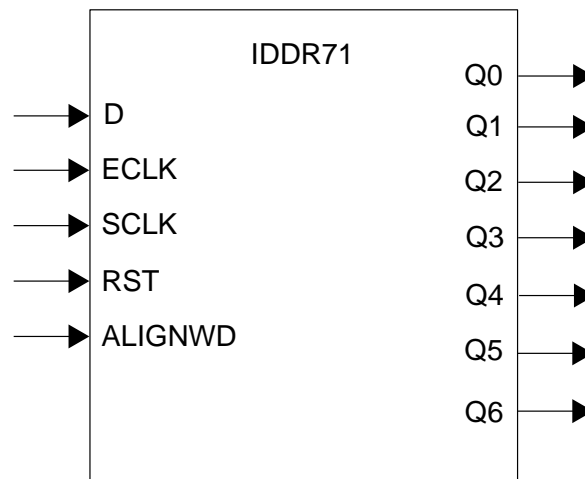
Figure 8.11. IDDR71 Primitive
