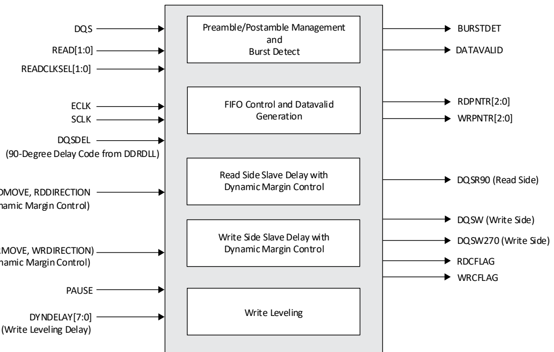
Figure 6.7. DQSBUF Block Functions
