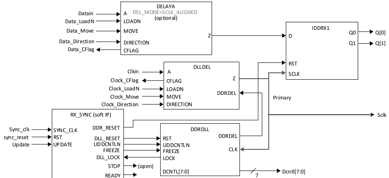
Figure 5.14. GDDR1_RX.SCLK.Aligned Interface (Dynamic Data/Clock Delay)
