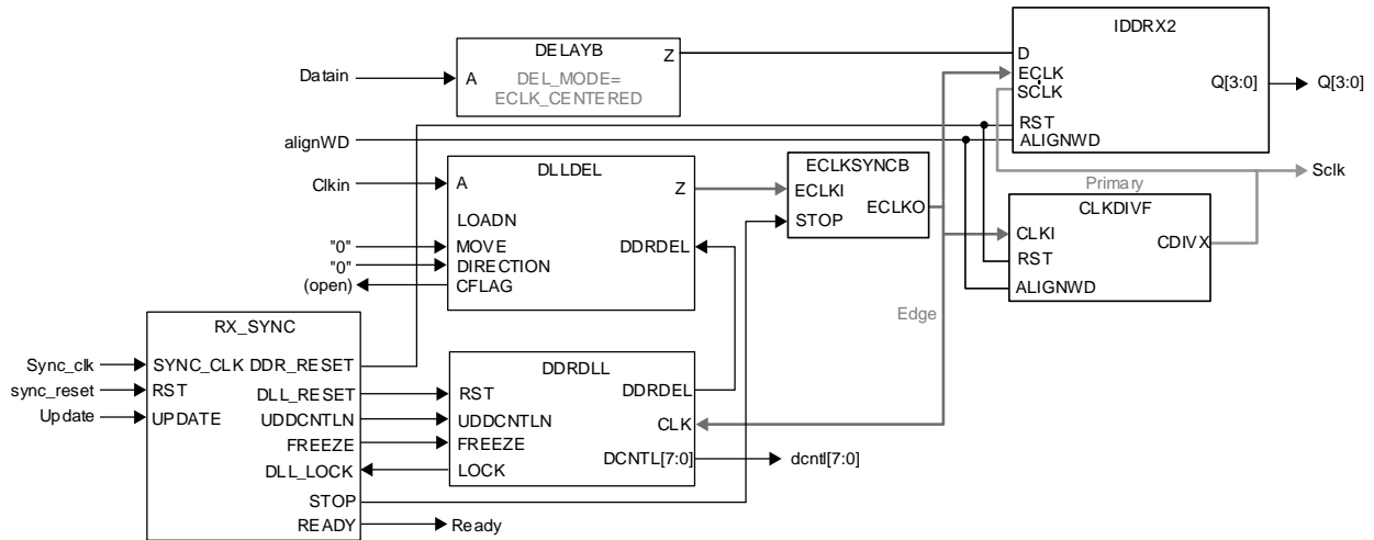
Figure 5.17. GDDR2_RX.ECLK.Aligned Interface (Static Delay)
