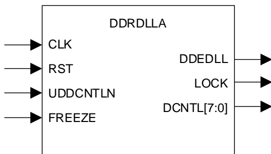
Figure 8.3. DDRDLA Primitive
