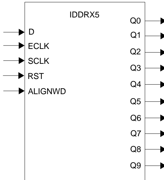
Figure 8.10. IDDRX5 Primitive
