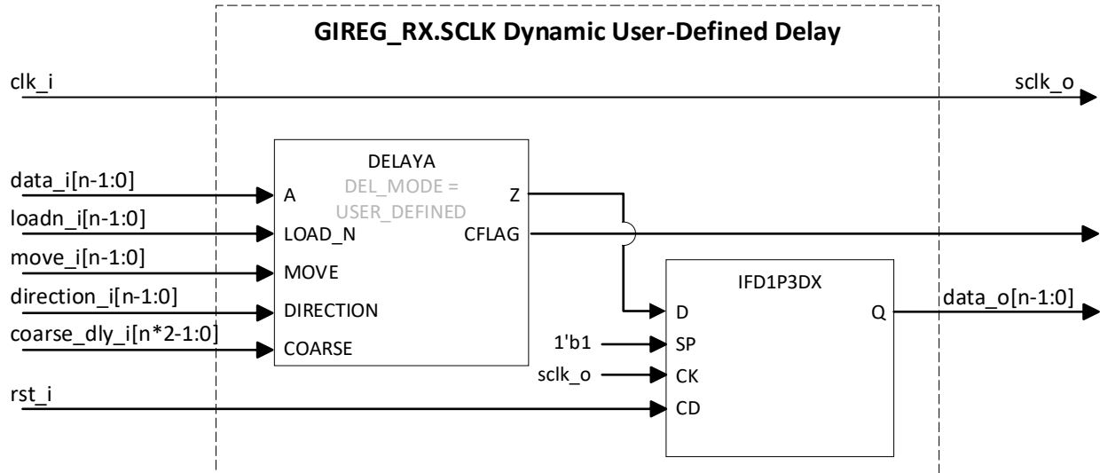
Figure 5.9. GIREG_RX.SCLK (Dynamic User-Defined Delay)
