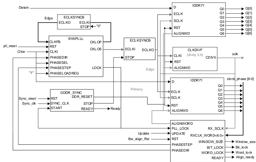
Figure 5.27. GDDR71_RX.ECLK Interface
