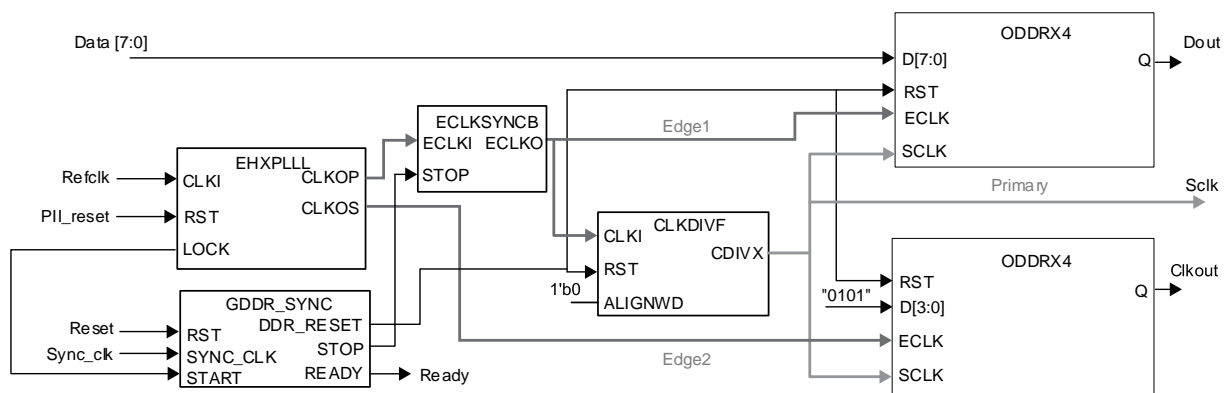
Figure 5.41. GDDR4_TX.ECLK.Centered Interface
