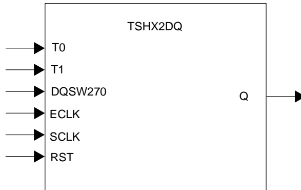
Figure 8.23. TSHX2DQ Primitive
