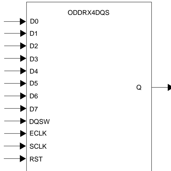
Figure 8.22. ODDR4DQS Primitive
