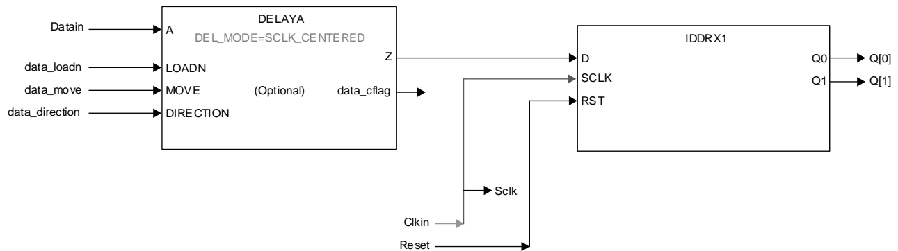
Figure 5.12. GDDR1_RX.SCLK.Centered Interface (Dynamic Data delay)
