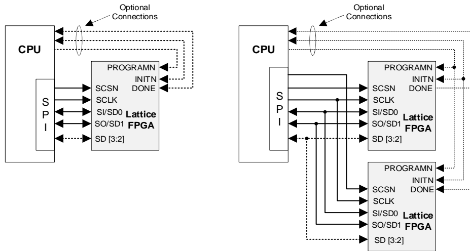
Figure 6.20. Nexus Slave SPI Port with CPU and Single or Multiple Devices
