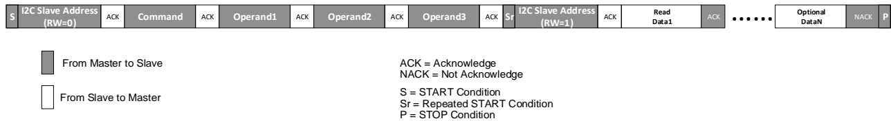
Figure 6.36. Typical I 2 C Read
