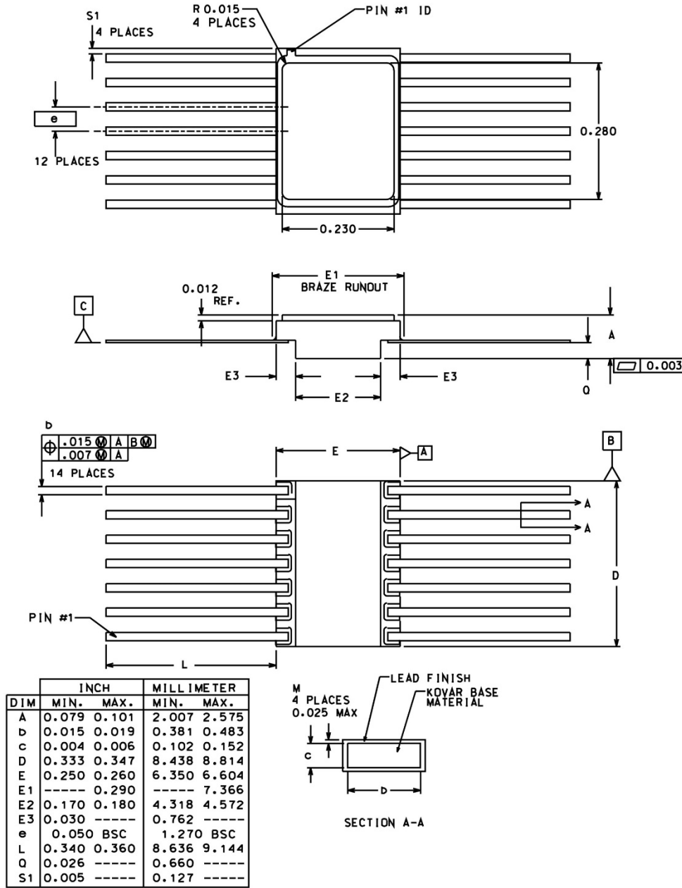
Figure 2: Figure 1. 14-Lead Flatpack
