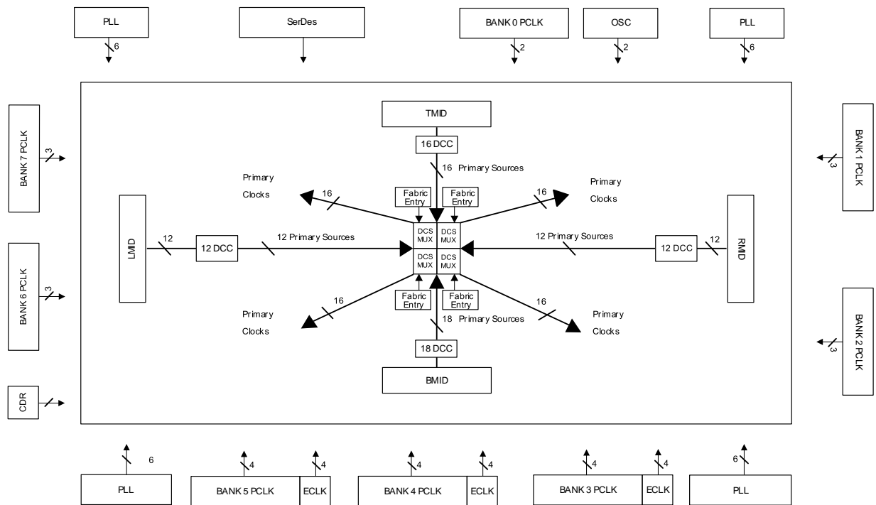
Figure 2.6 Clocking Network
