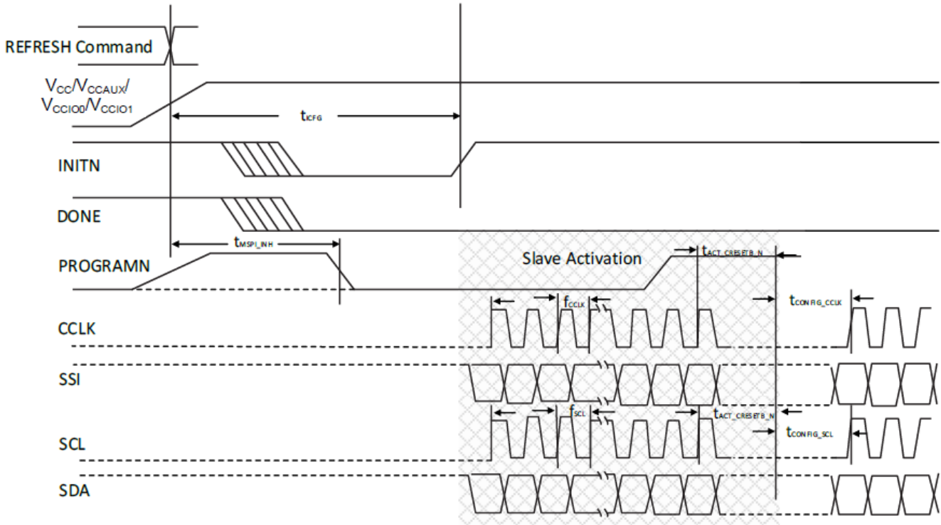
Figure 3.15. Slave SPI/ I 2 C /I3C POR/REFRESH Timing
