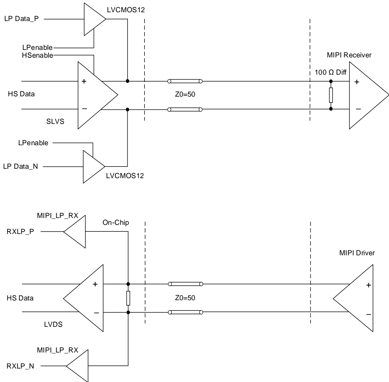
Figure 3.6. MIPI Interface
