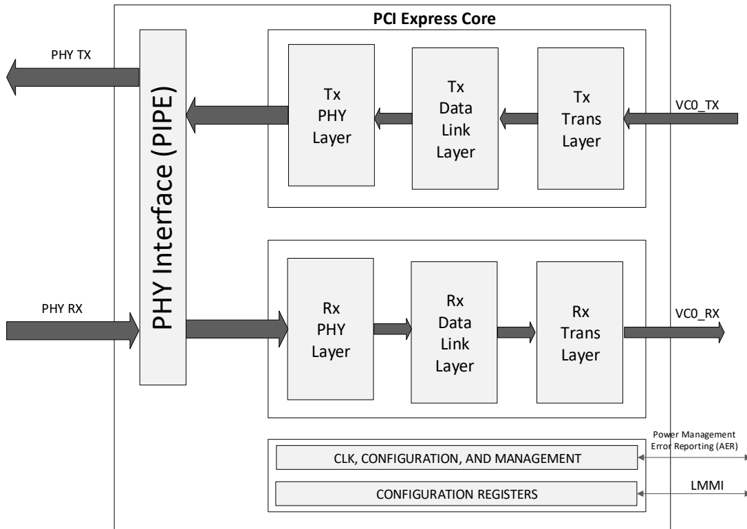
Figure 2.33 PCIe Core
