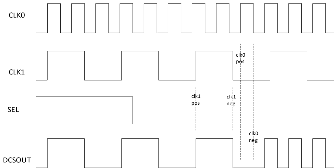
Figure 2.9 DCS Waveforms
