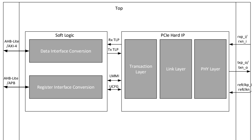
Figure 2.34 PCIe Soft IP Wrapper
