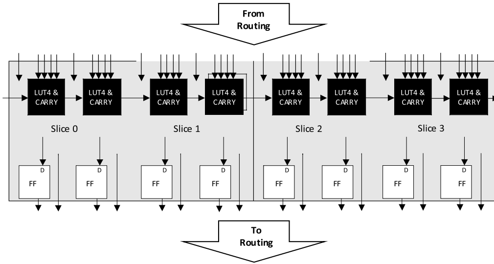
Figure 2.2 PFU Diagram
