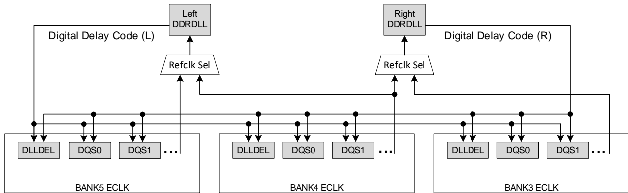
Figure 2.11 CertusPro-NX-RT DDRDLL Architecture
