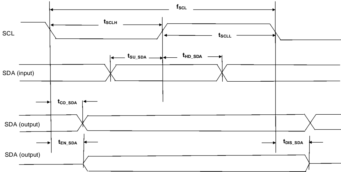
Figure 3.20. I 2 C /I3C Configuration Timing
