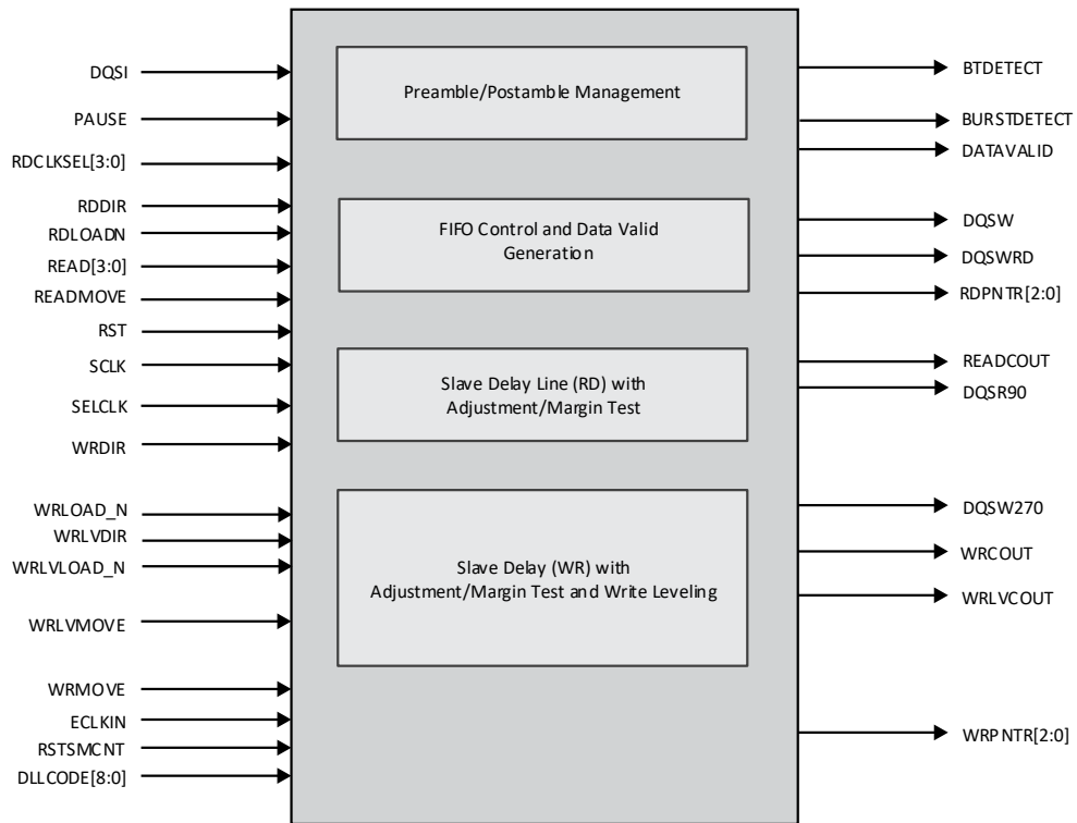
Figure 2.25 DQS Control and Delay Block (DQSBUF)
