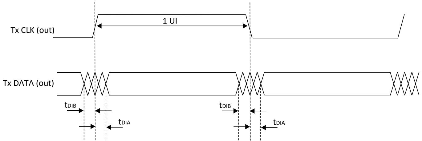
Figure 3.10. Transmit TX.CLK.Aligned Waveforms
