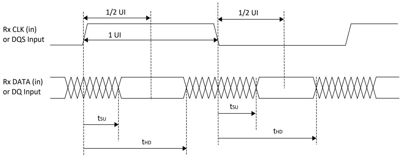
Figure 3.8. Receiver RX.CLK.Aligned and DDR Memory Input Waveforms
