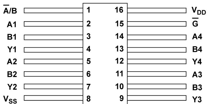
16-Lead Flatpack Top View
