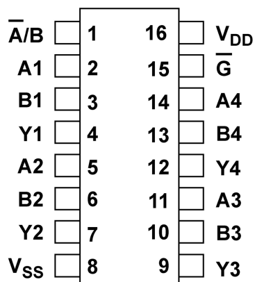
16-Pin DIP Top View
