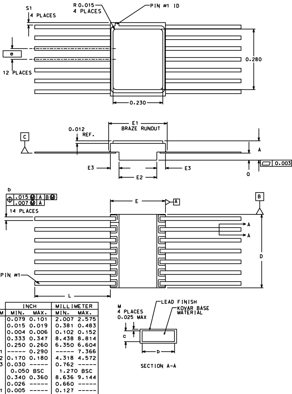
Figure 1. 14-Lead Flatpack
