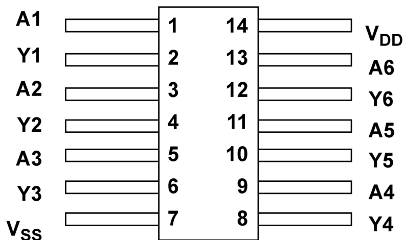
14-Lead Flatpack Top View
