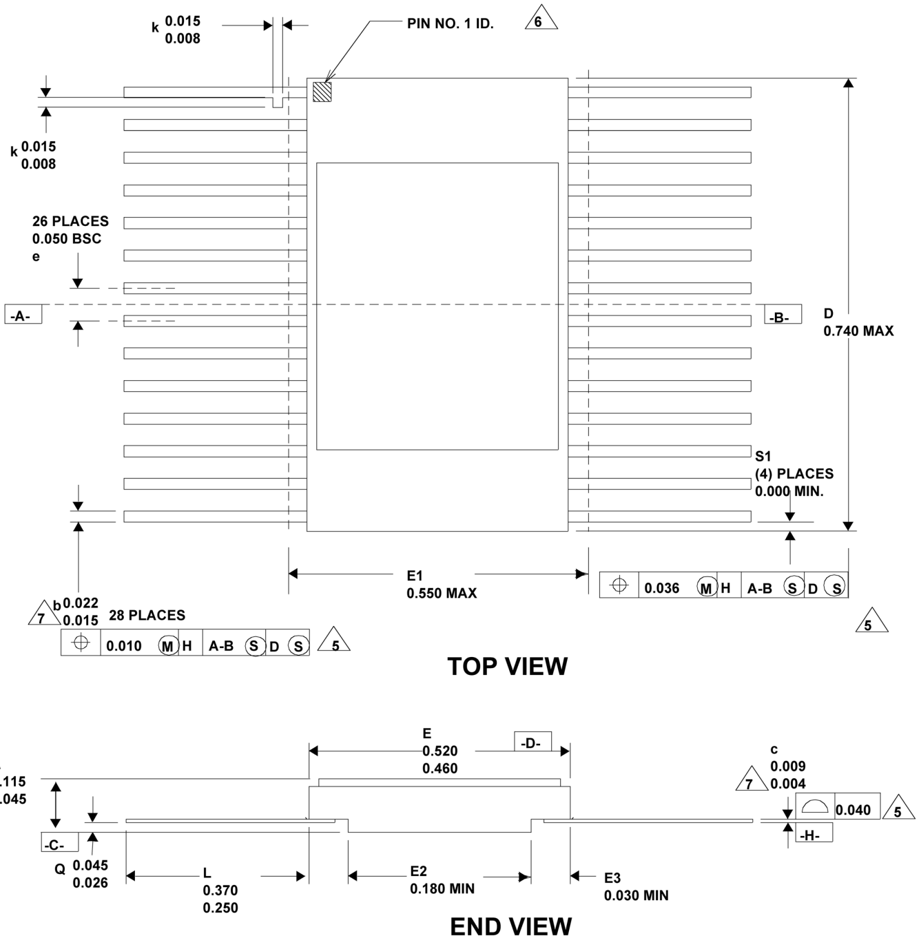
Figure 5. 28-Lead 50-mil Center Flatpack (0.490 x 0.74)
