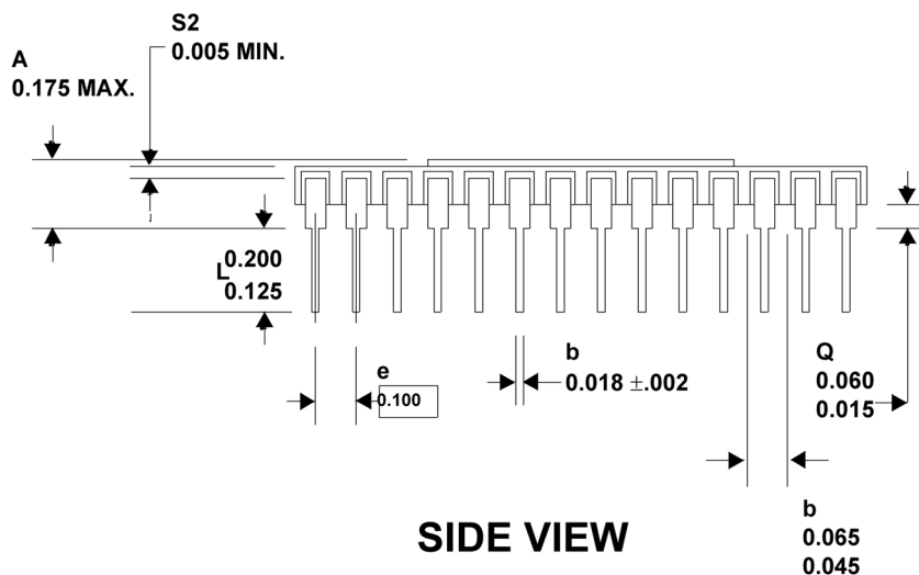
Figure 4. 28-Pin 100-mil Center DIP (0.600 × 1.4)
