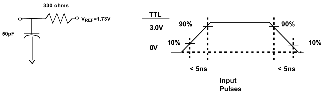
Figure 3. AC Test Loads and Input Waveforms
