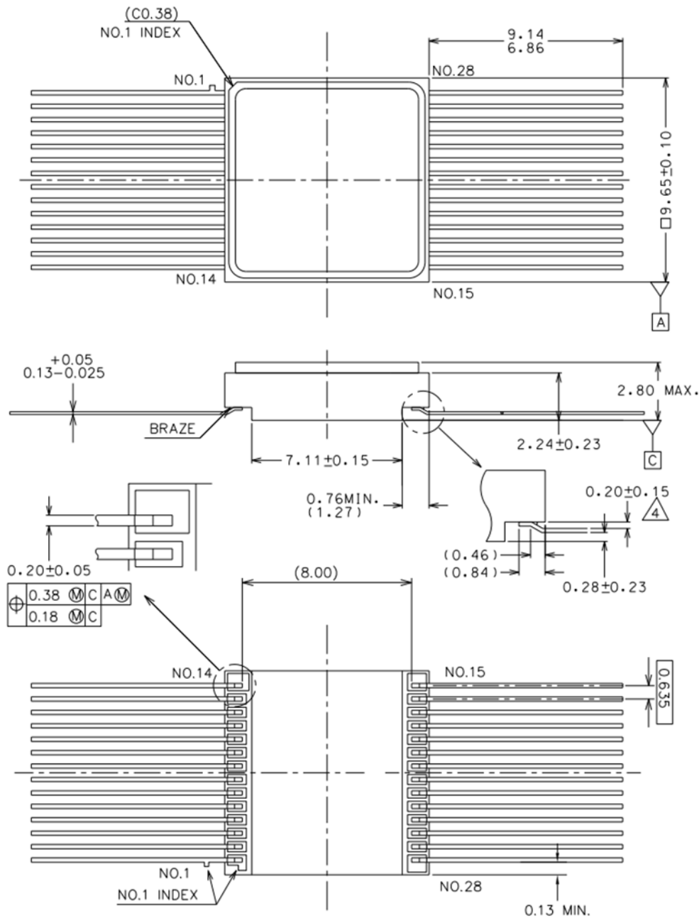
Figure 11. 28-pin Flatpack
