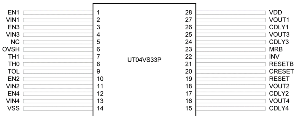
Figure 2. UT04VS33P Pin Configuration
