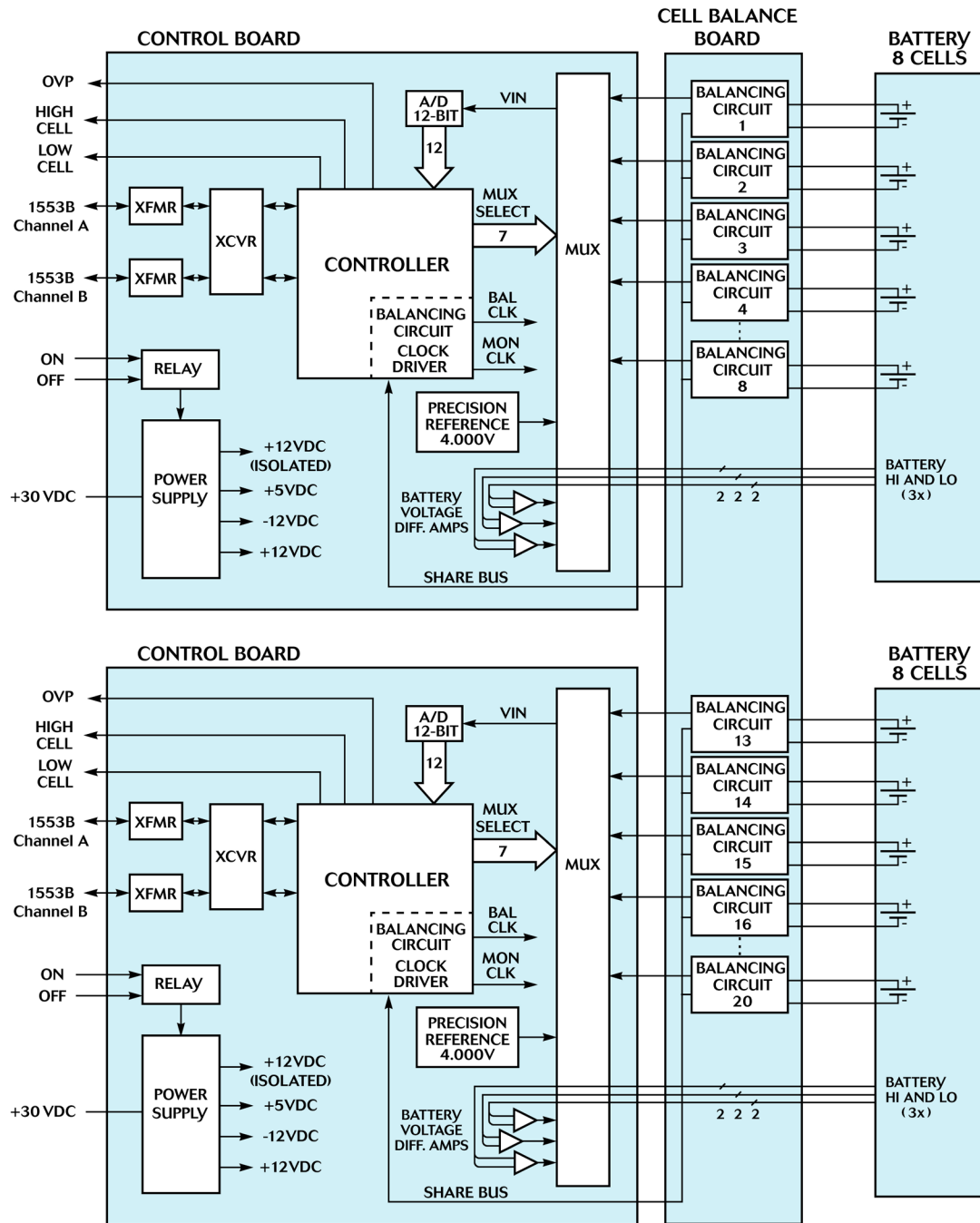
Block Diagram
