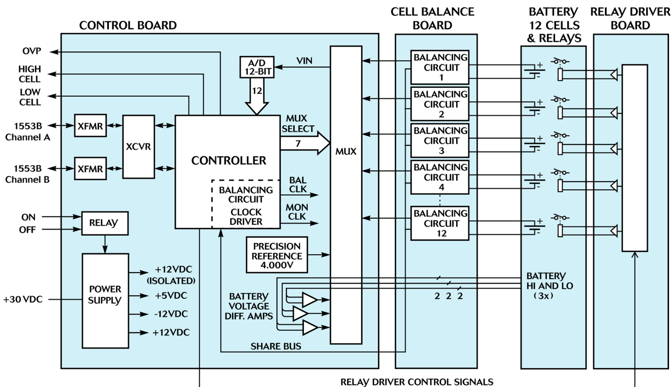
Block Diagram
