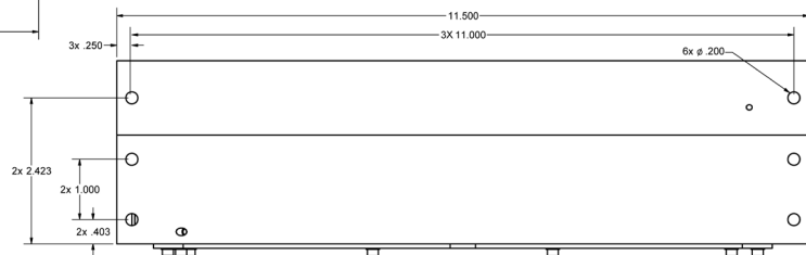
Outline
