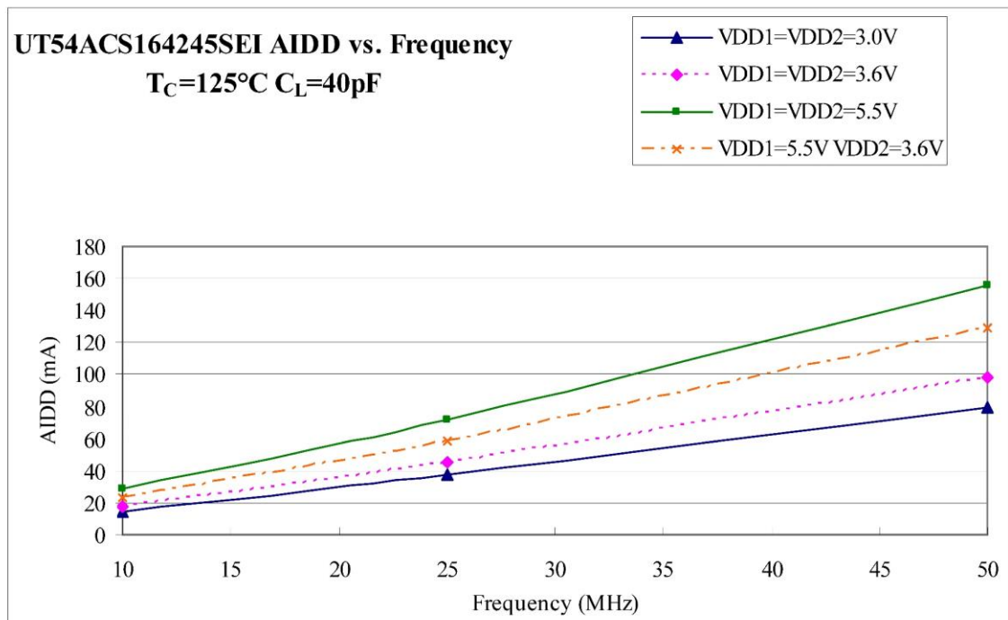
Figure 1. AIDD Values for 125°C with all 16 outputs switching
