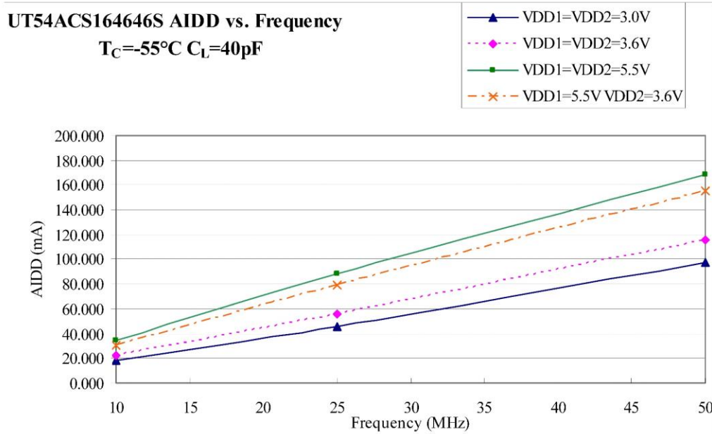
Figure 9. AIDD Values for -55°C with all 16 outputs switching
