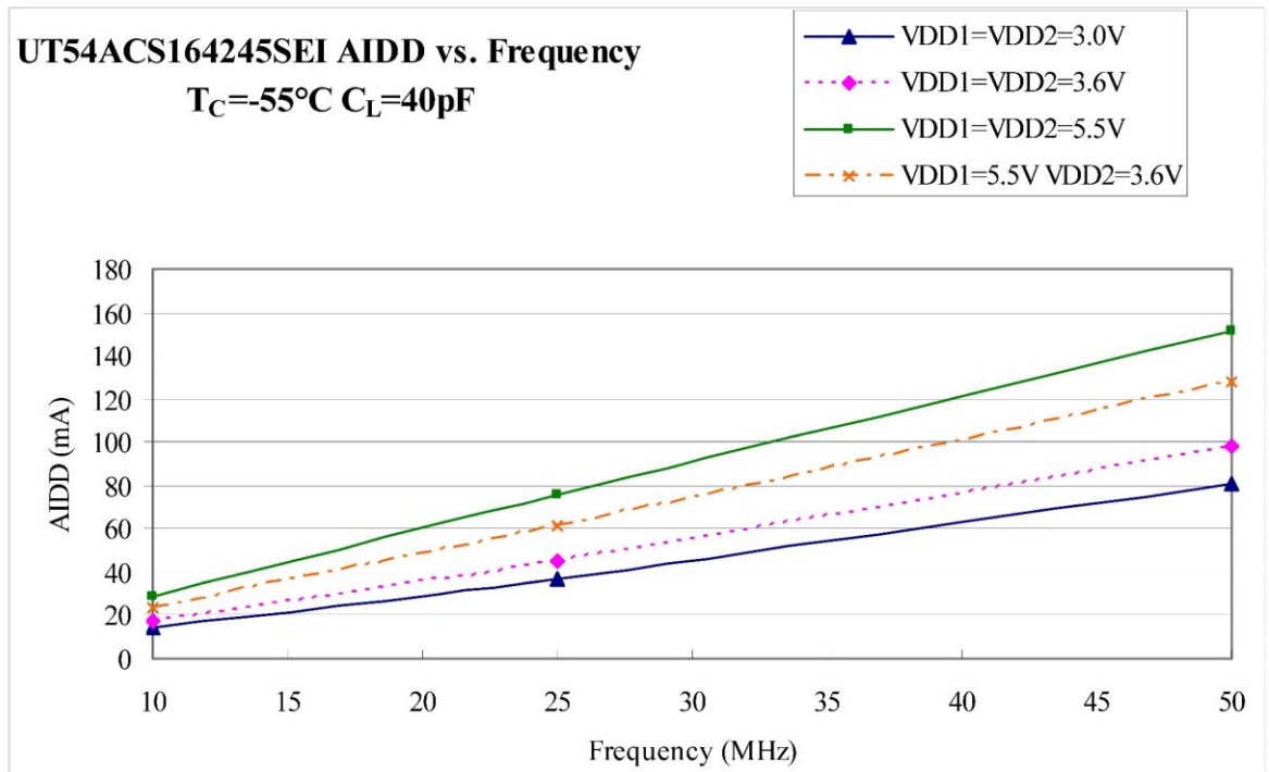
Figure 3. AIDD Values for -55°C with all 16 outputs switching
