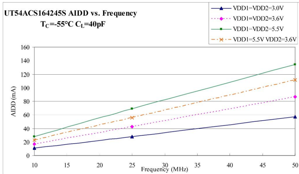
Figure 6. AIDD Values for -55°C with all 16 outputs switching
