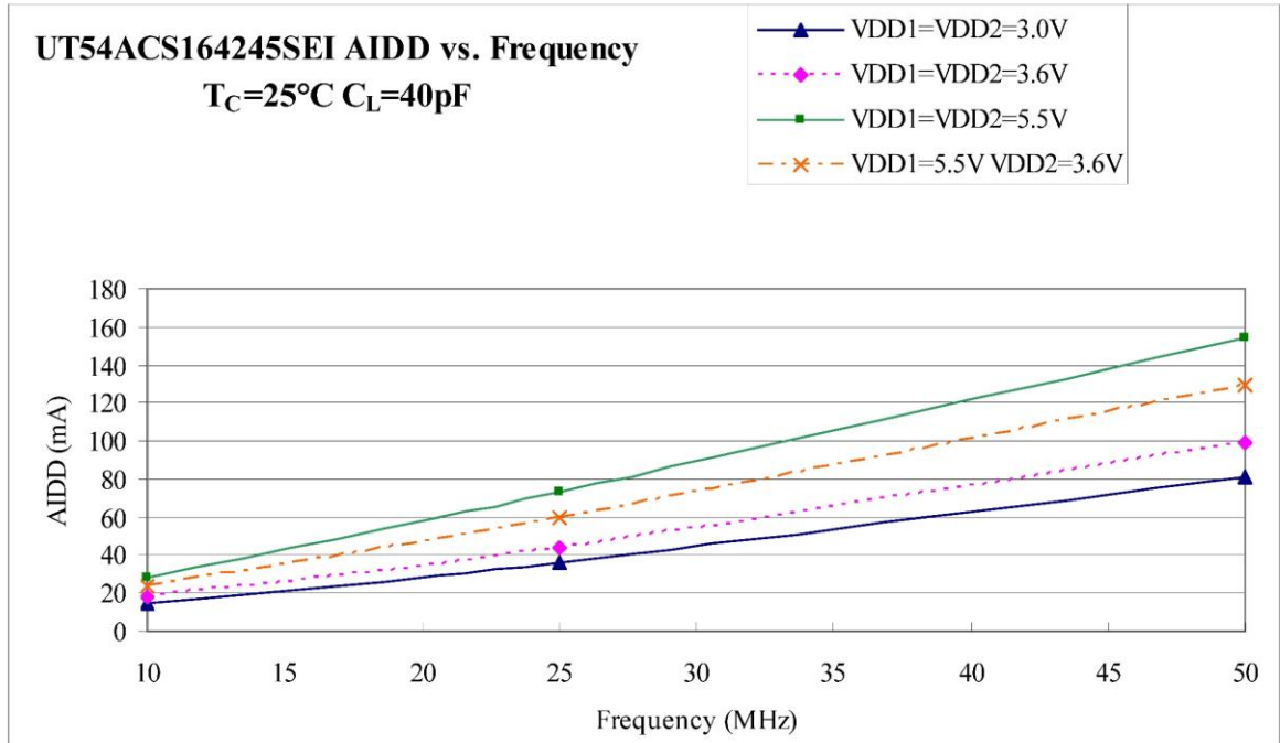
Figure 2. AIDD Values for 25°C with all 16 outputs switching
