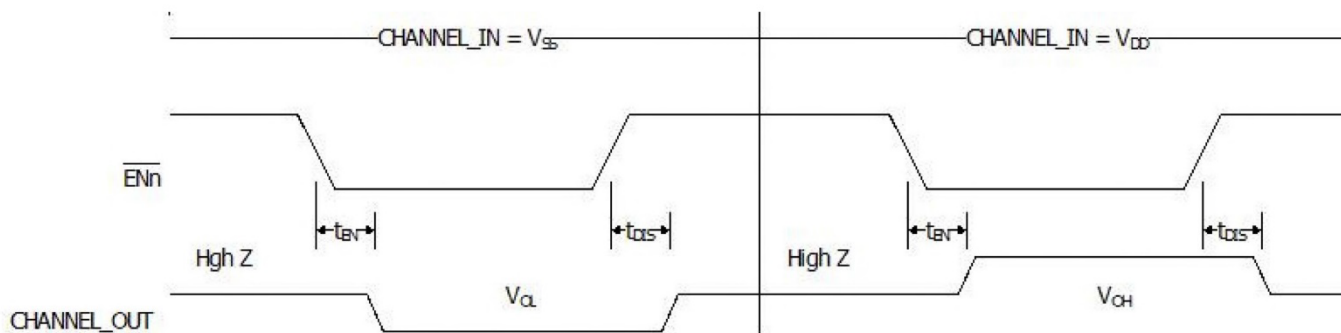
Figure 4: Enable Timing
