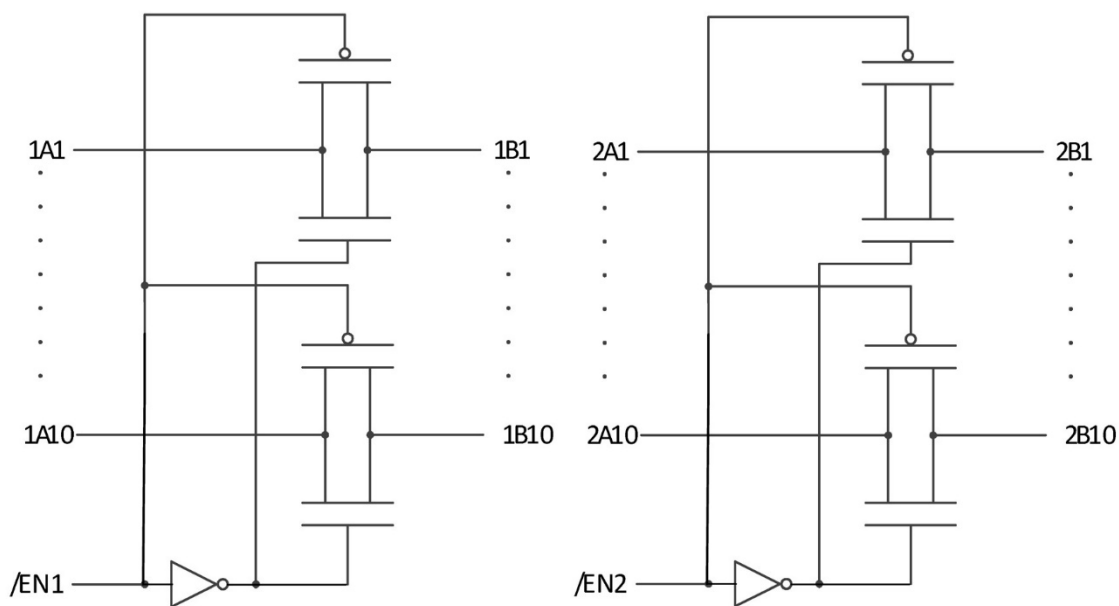
Figure 1: 20-bit Bus Switch Block Diagram
