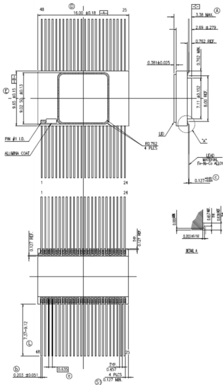
Figure 6: 48-Lead Flatpack
