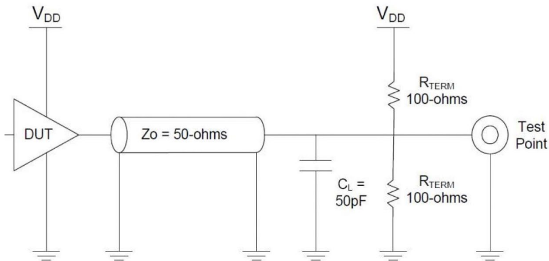
Figure 5. Standard Test Load
