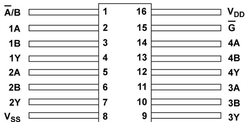
Figure 1: 16-Lead Flatpack Top View
