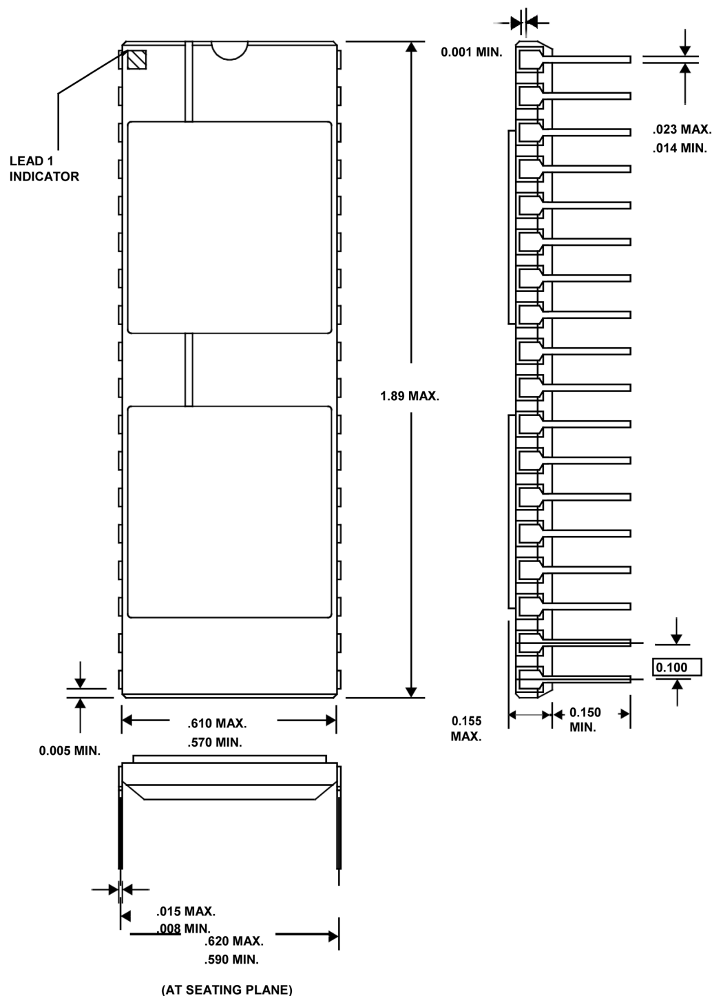
Figure 14. 36-Pin Side-Brazed DIP, Dual Cavity
