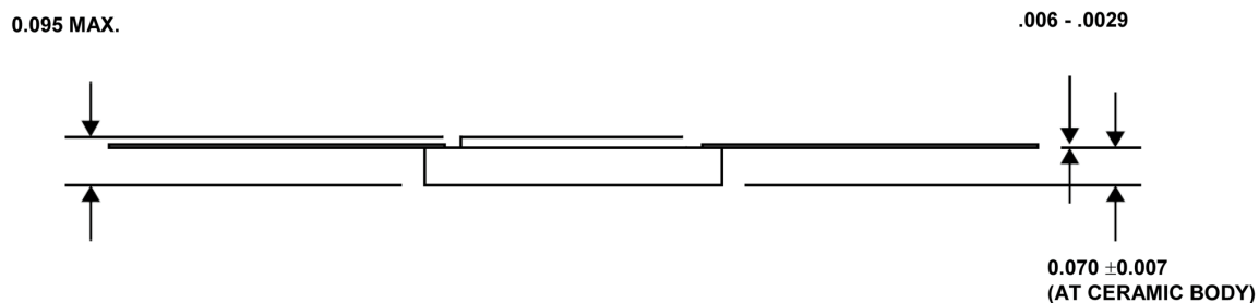
Figure 15. 24-Lead Flatpack, Top Brazed, Dual Cavity (50-mil lead spacing)
