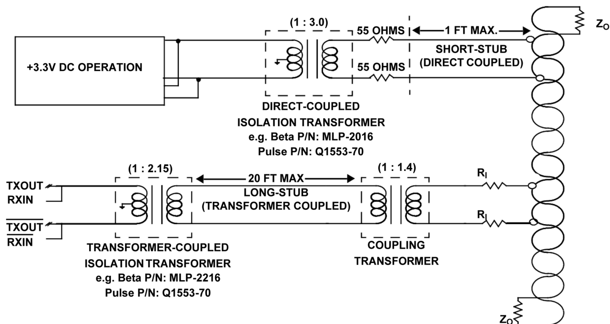
Figure 5. Bus Coupling Configuration
