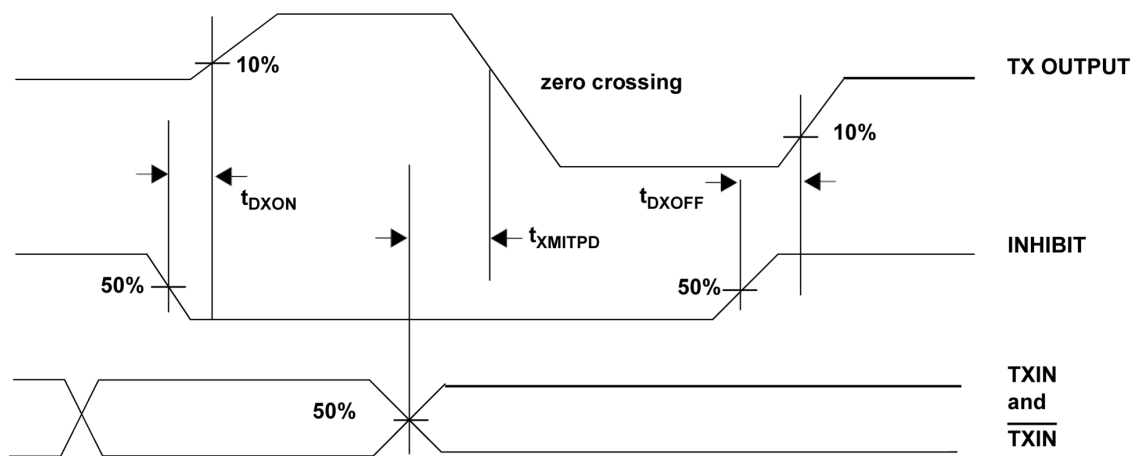
Figure 12. Transmitter Timing
