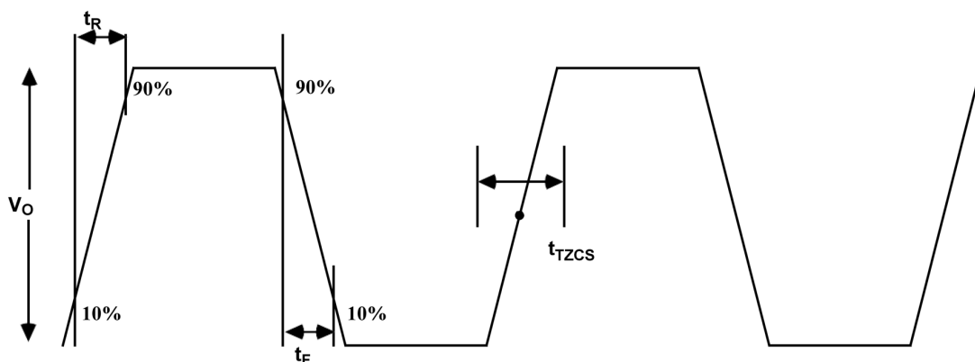
Figure 10. Transmitter Output Zero Crossing Stability, Rise Time, Fall Time ( t_{ZCS} , t_R , t_F )
