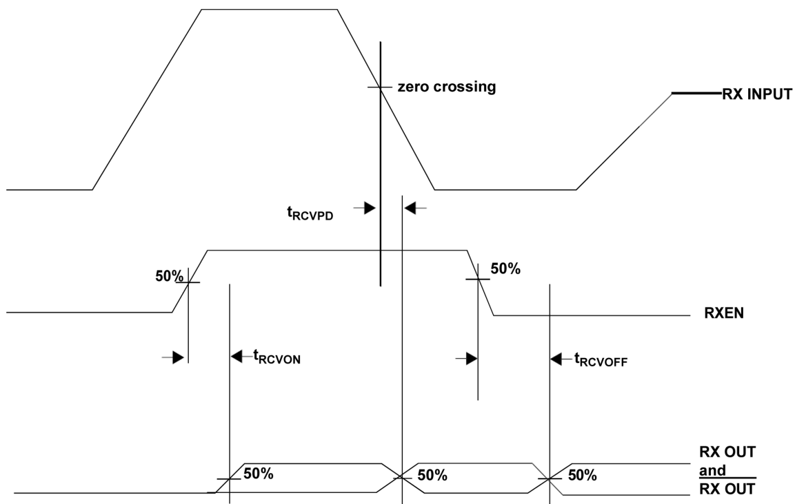
Figure 13. Receiver Timing
