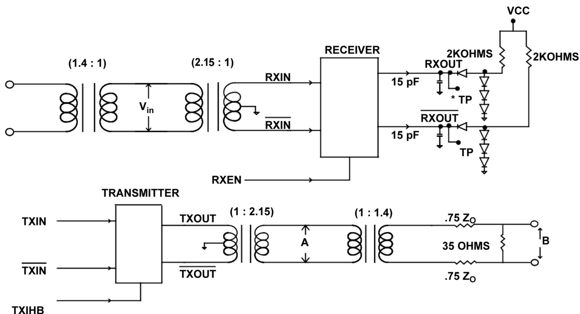
Figure 7. Transformer Coupled Transceiver with Load
